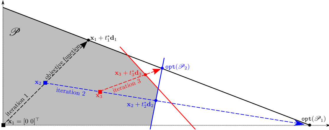
Figure 1: The first 3 iterations of the Projective Cutting-Planes on an LP with 2 variables. At the first iteration, the projection sub-problem projects \mathbf{x}_1 = \mathbf{0} = [0 \ 0]^\top along the objective function, as depicted by the black dashed arrow. At iteration \text{it} = 2 , the midpoint \mathbf{x}_2 of this black arrow is projected towards the optimal outer solution \text{opt}(\mathcal{P}_1) — at iteration 1, the outer approximation \mathcal{P}_1 \supset \mathcal{P} only contains the largest triangle. This generates a second facet (blue solid line) that is added to the facets of \mathcal{P}_1 to construct \mathcal{P}_2 . The third projection is represented by the short arrow in red.
