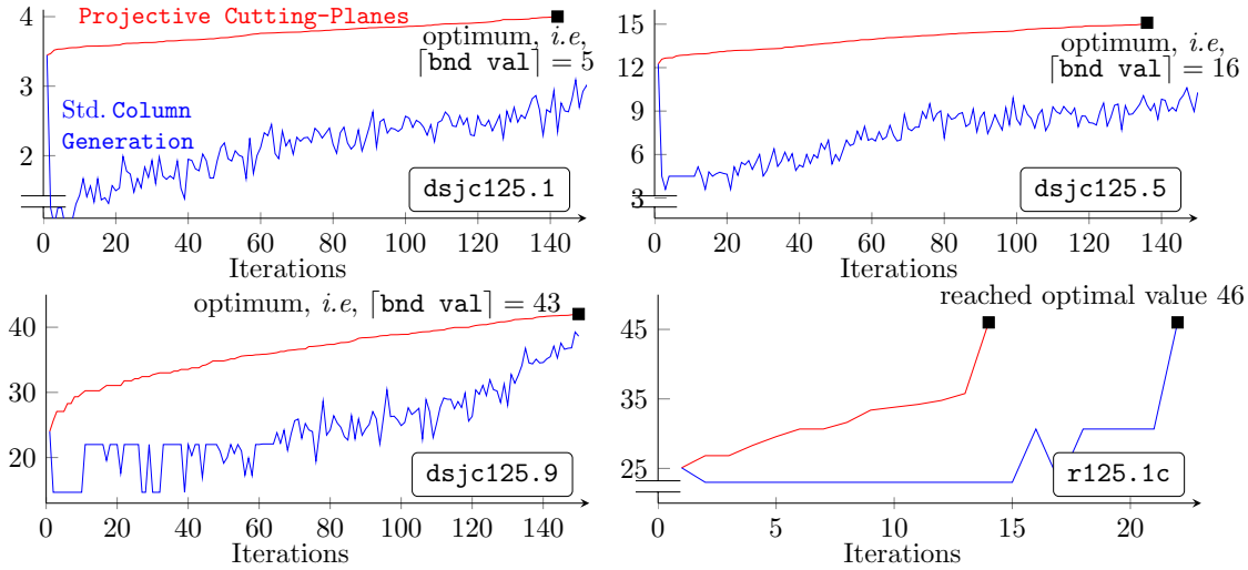
Figure 3: The lower bounds generated along the iterations by Projective Cutting-Planes (in red) and resp. Column Generation (in blue) on 4 instances.
