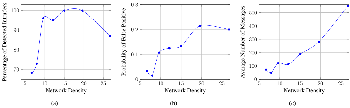
Fig. 1. Percentage of Detected Intruders, False Positive Rate and Traffic Depending on the Network Density
