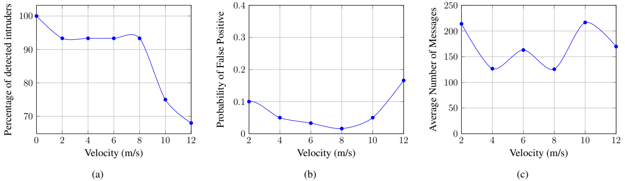
Fig. 2. Intruder Detection and False Positive Rate and Traffic According to the Mobility
