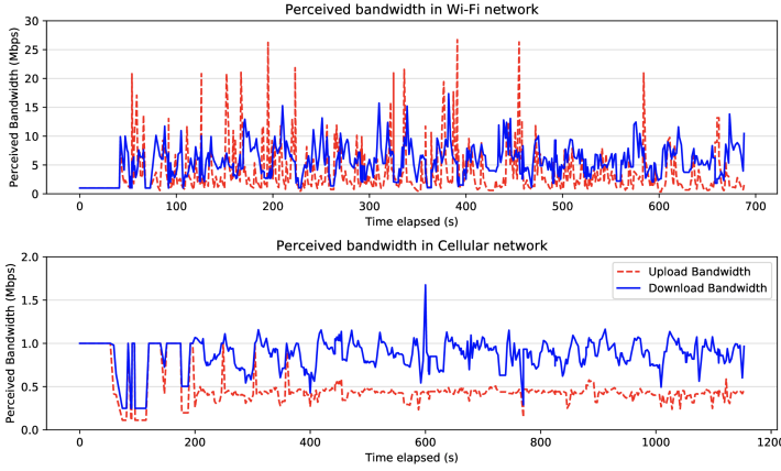
Fig. 9. Change in perceived bandwidth over elapsed time.
