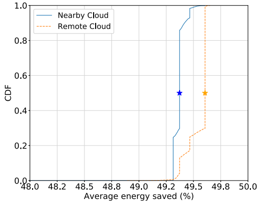
Fig. 8. Energy gain cumulative distribution (simulation).
