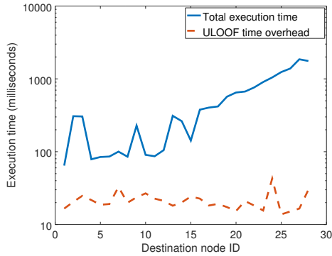
Fig. 13. Overhead caused by the offloading framework.
