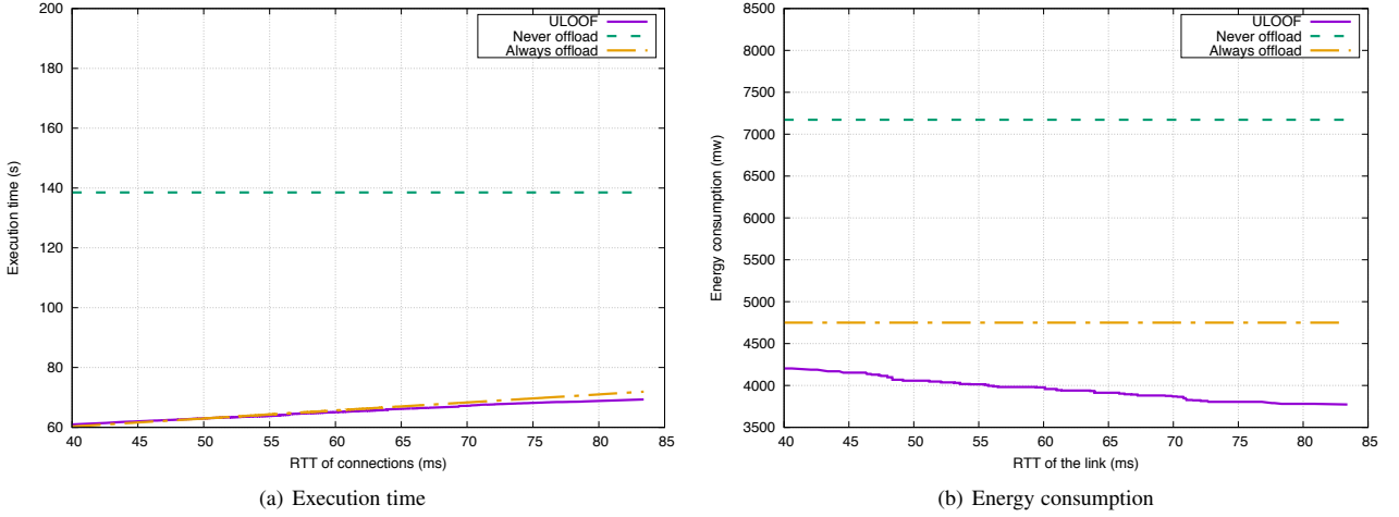
Fig. 6. Performance as a function of the RTT (simulation).
