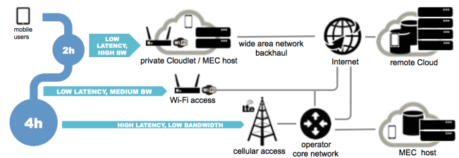
Fig. 1. Mobile computation offloading scenarios
