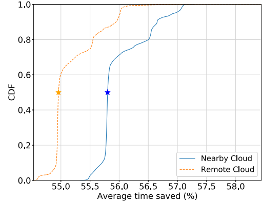
Fig. 7. Execution time gain cumulative distribution (simulation).
