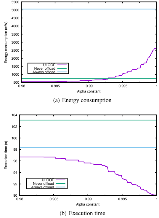
Fig. 14. ULOOF performance as a function of \alpha (CityRoute).
