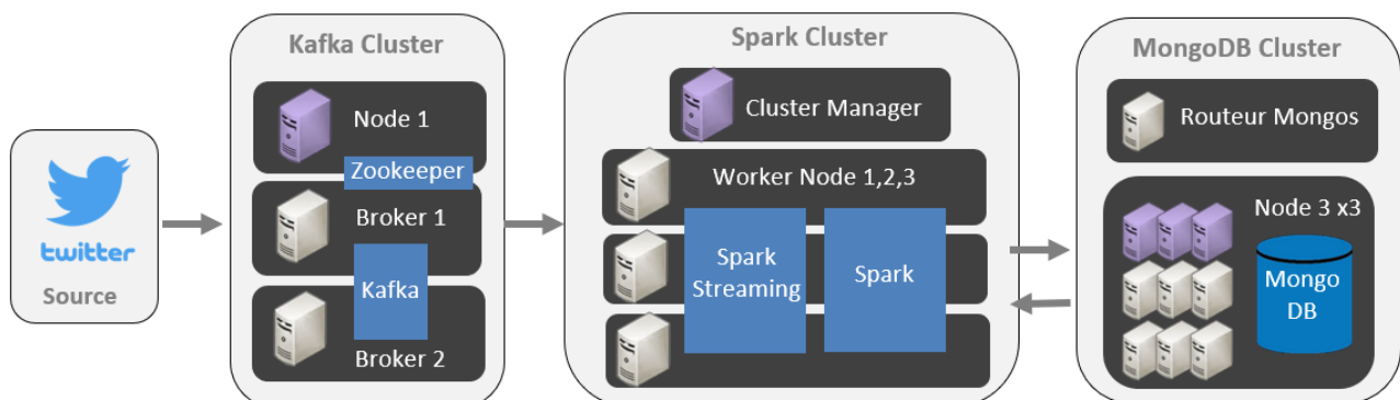
Figure 22: Architecture Technique du projet
