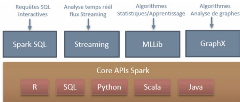
Figure 26: Composants de la stack technique de Spark
