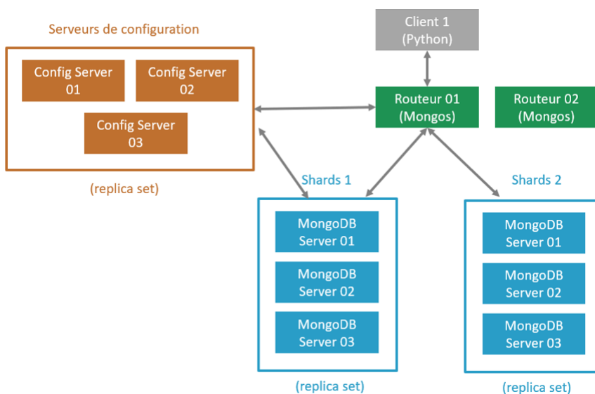
Figure 30: Architecture MongoDB
