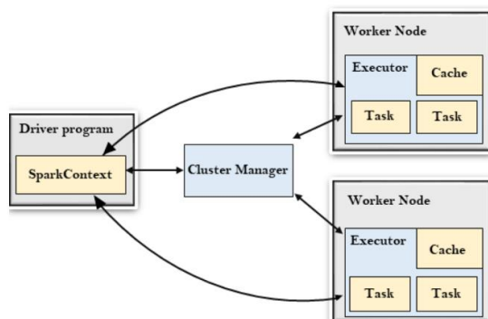
Figure 27: Architecture de Spark
