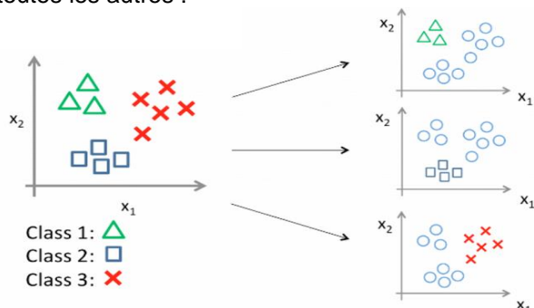
Figure 15 : Algorithme One-vs-Rest
