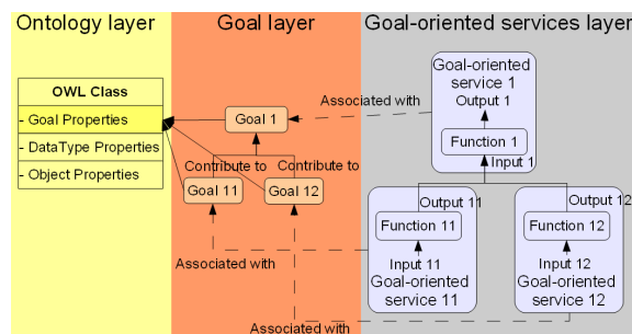
Figure 1: The meta-model.
