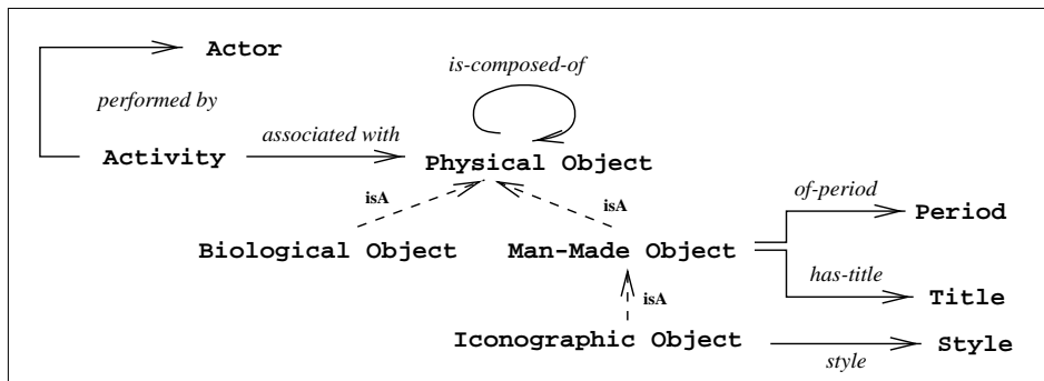
Figure 3: A simple cultural ontology.
