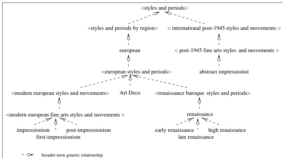
Figure 5: Part of the Art & Architecture Thesaurus hierarchy Styles & Periods which collects all styles, periods and movements of Art in the western world.
