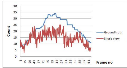
Figure 4: People count in the individual frames from PETS sequence S1.L1 using single view.
