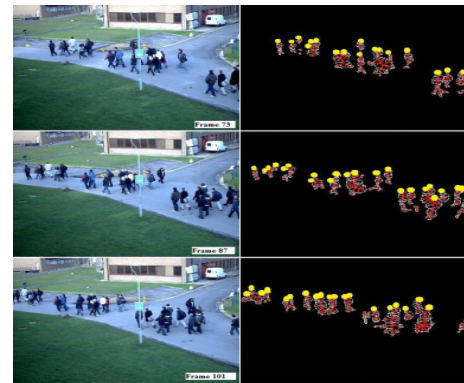
Figure 6: Sample head detection results on PETS data in image plane View1.
