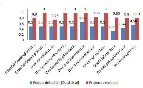
Figure 8: Counting people accuracy for the different group of humans.
