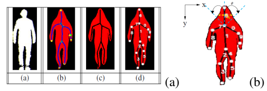
Figure 2: (a) Skeleton graph computing. (b) Head detection.
