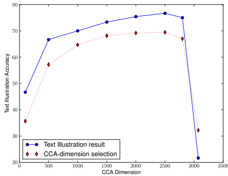
Figure 1: CCA_{cap} result and dimension selection
