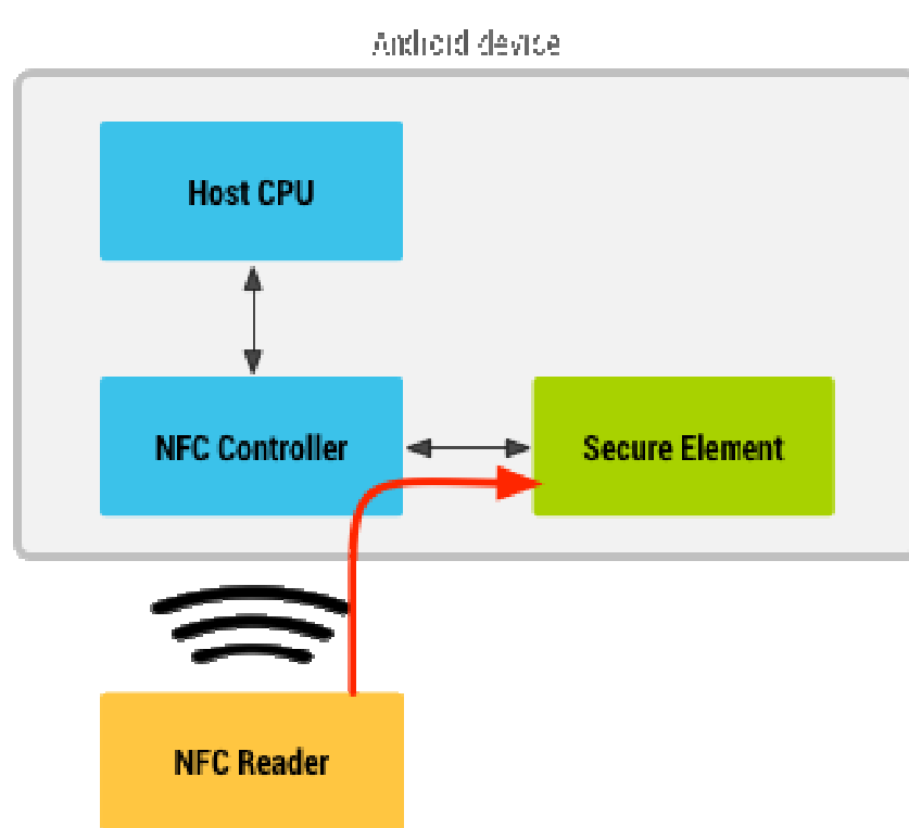
NFC card emulation with a secure element
